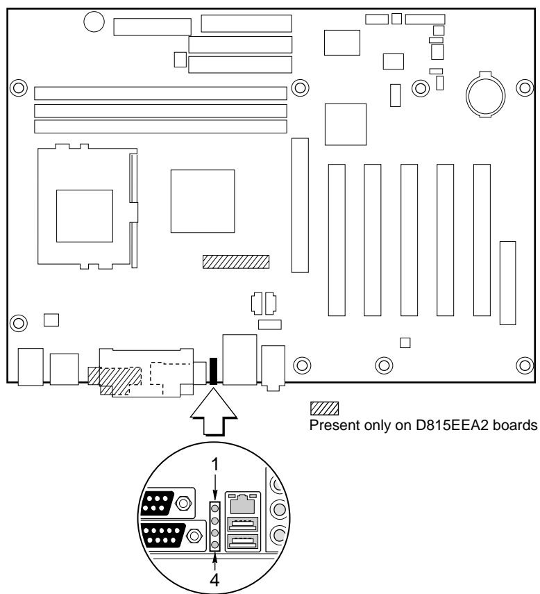
Figure 26. Diagnostic LEDs
